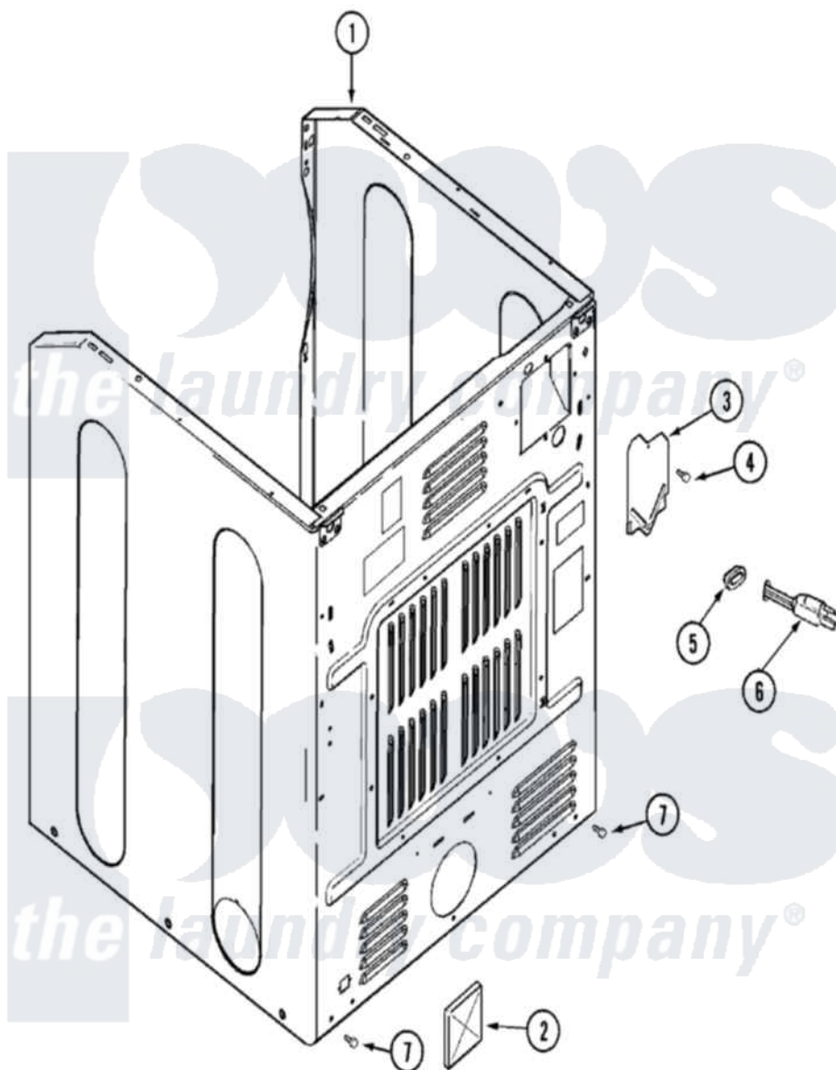
Maytag Residential Maytag MDE6200AYQ Dryer Parts Parts Diagram 02 - CABINET-REAR Click on the part number to view part
