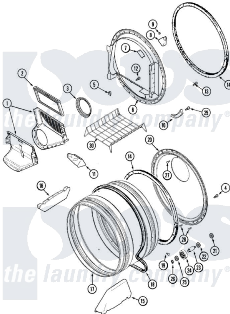
Maytag Residential Maytag MDE6200AYW Dryer Parts Parts Diagram 07 - TUMBLER Click on the part number to view part
