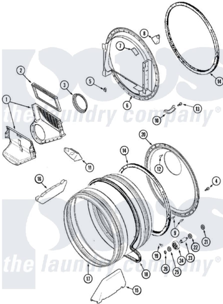
Maytag Residential Maytag MDE6460AYW Dryer Parts Parts Diagram 07 - TUMBLER Click on the part number to view part
