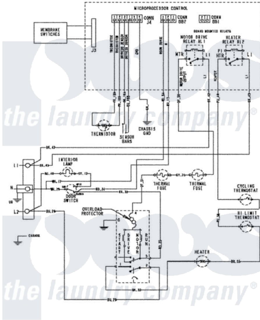
Maytag Residential Maytag MDE6800AYW Dryer Parts Parts Diagram 06 - WIRING INFORMATION Click on the part number to view part
