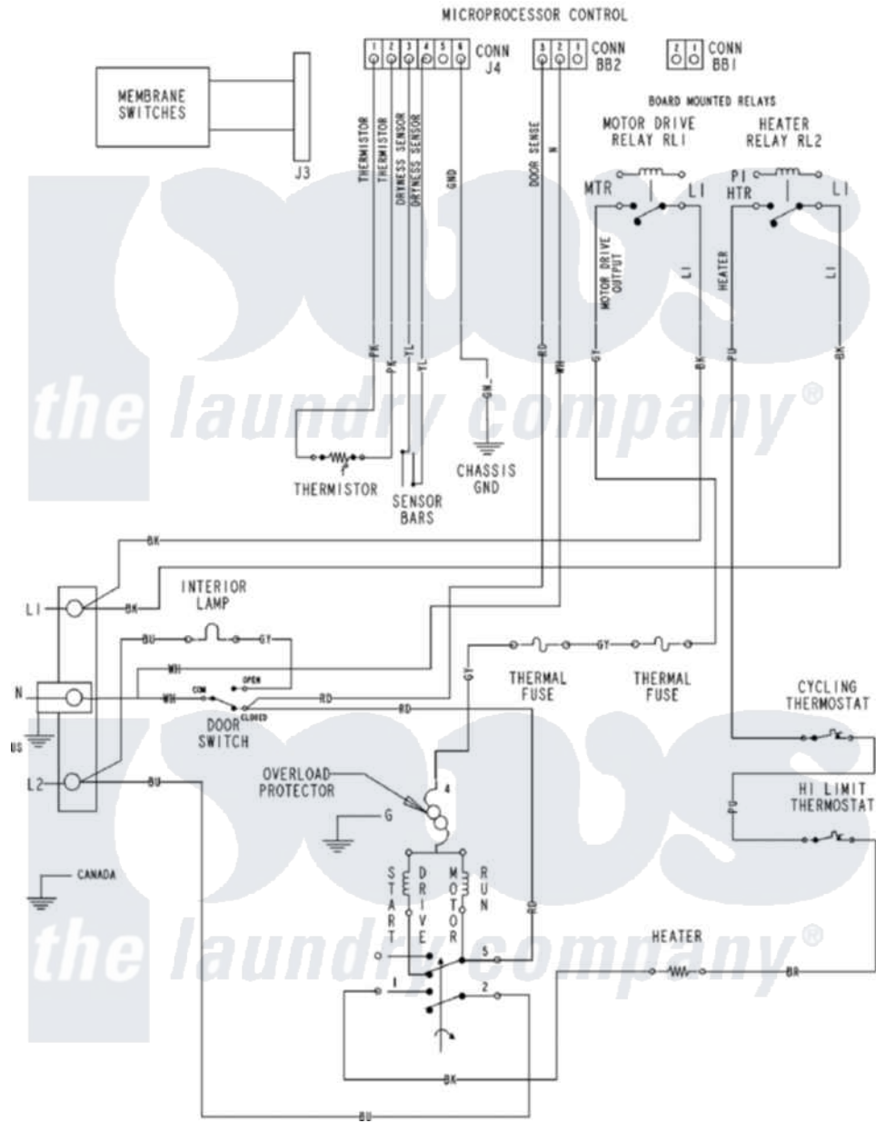
Maytag Residential Maytag MDE6800AYW Dryer Parts Diagram 07 - WIRING INFORMATION Click on the part number to view part
