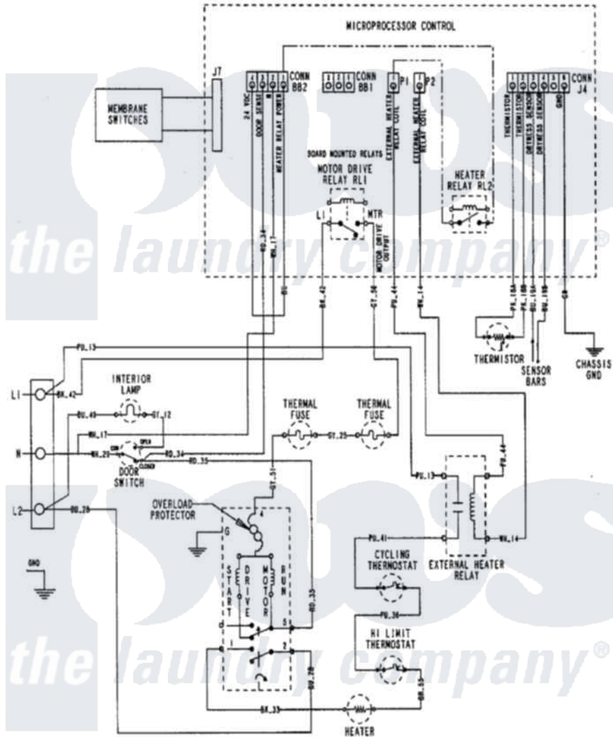
Maytag Residential Maytag MDE7500AZQ Dryer Parts Parts Diagram 08 - WIRING INFORMATION (AT SERIES 34)
