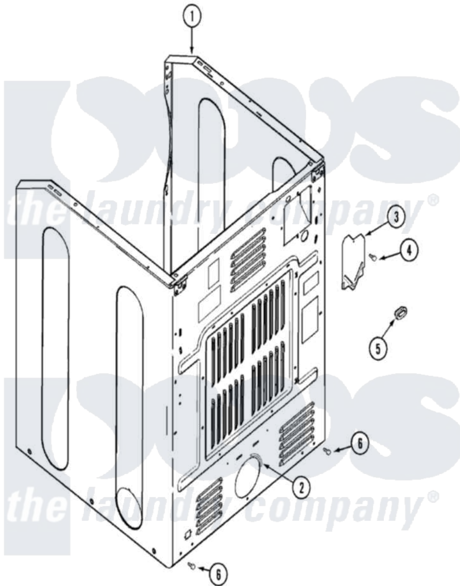
Maytag Residential Maytag MDE7500AZW Dryer Parts Parts Diagram 01 - CABINET-REAR Click on the part number to view part
