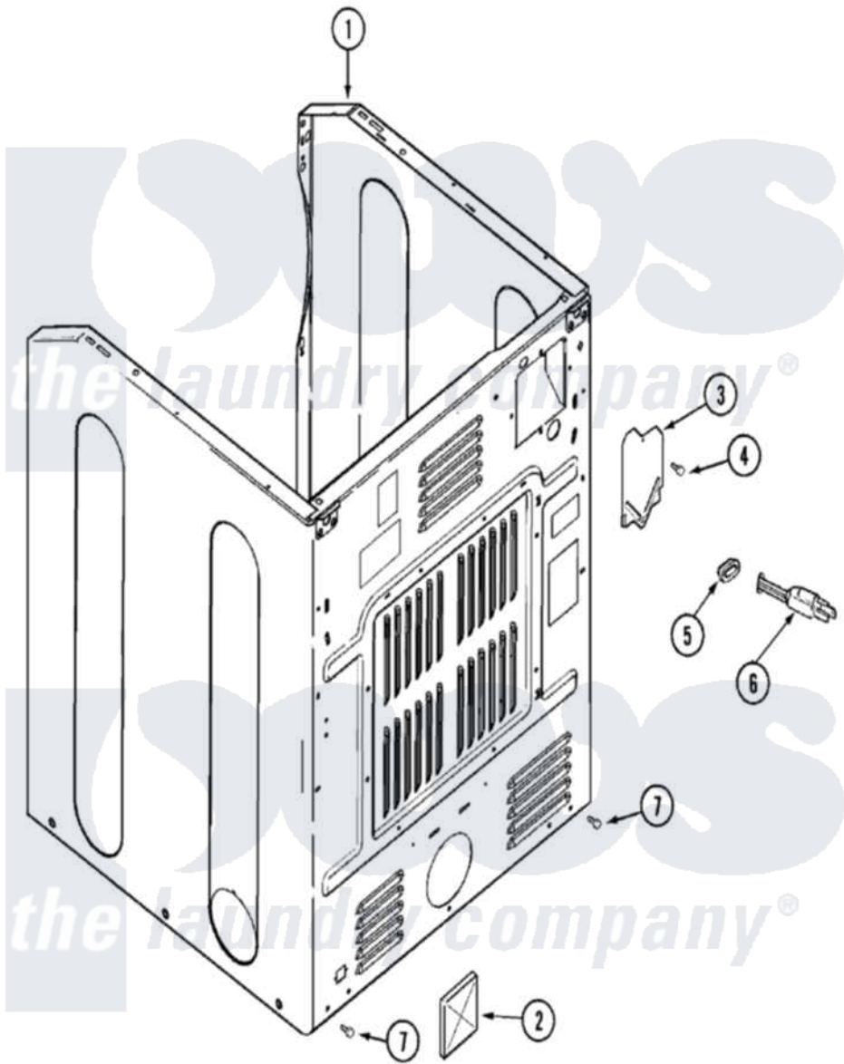
Maytag Residential Maytag MDE7600AYQ Dryer Parts Parts Diagram 02 - CABINET-REAR Click on the part number to view part
