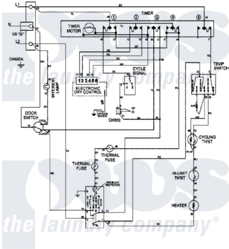
Maytag Residential Maytag MDE7657BYW Dryer Parts Parts Diagram 08 - WIRING INFORMATION Click on the part number to view part
