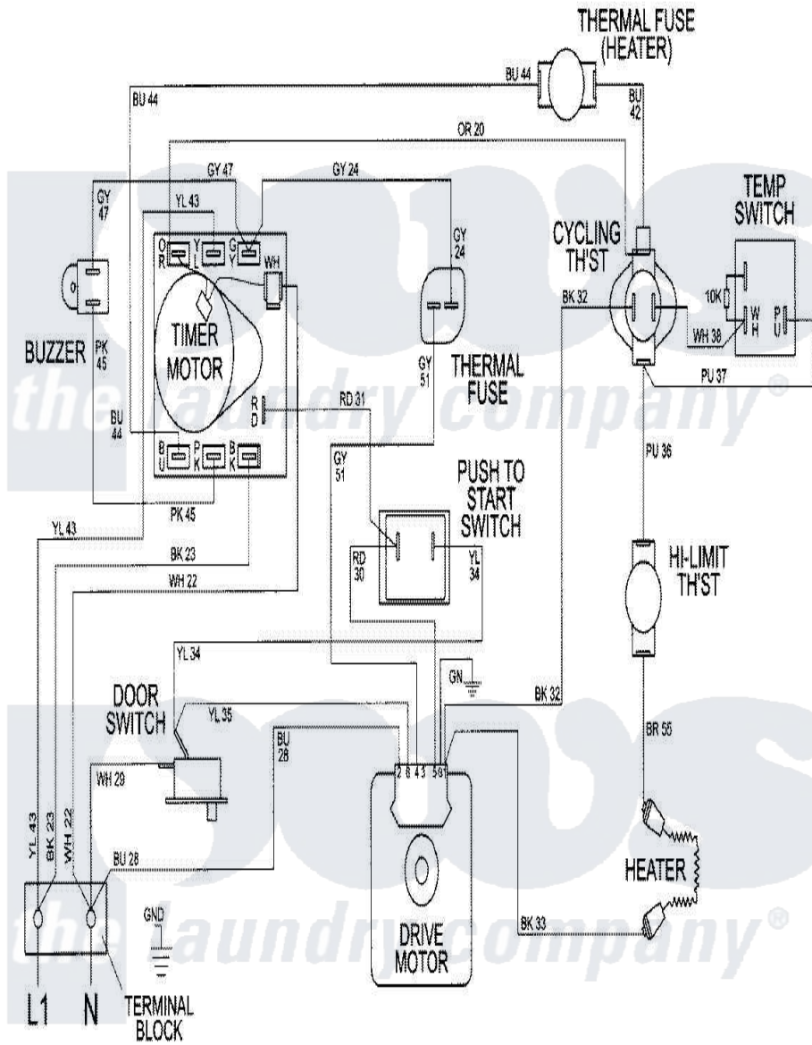
Maytag Residential Maytag MDE8426AAW Dryer Parts Parts Diagram 08 - WIRING INFORMATION Click on the part number to view part
