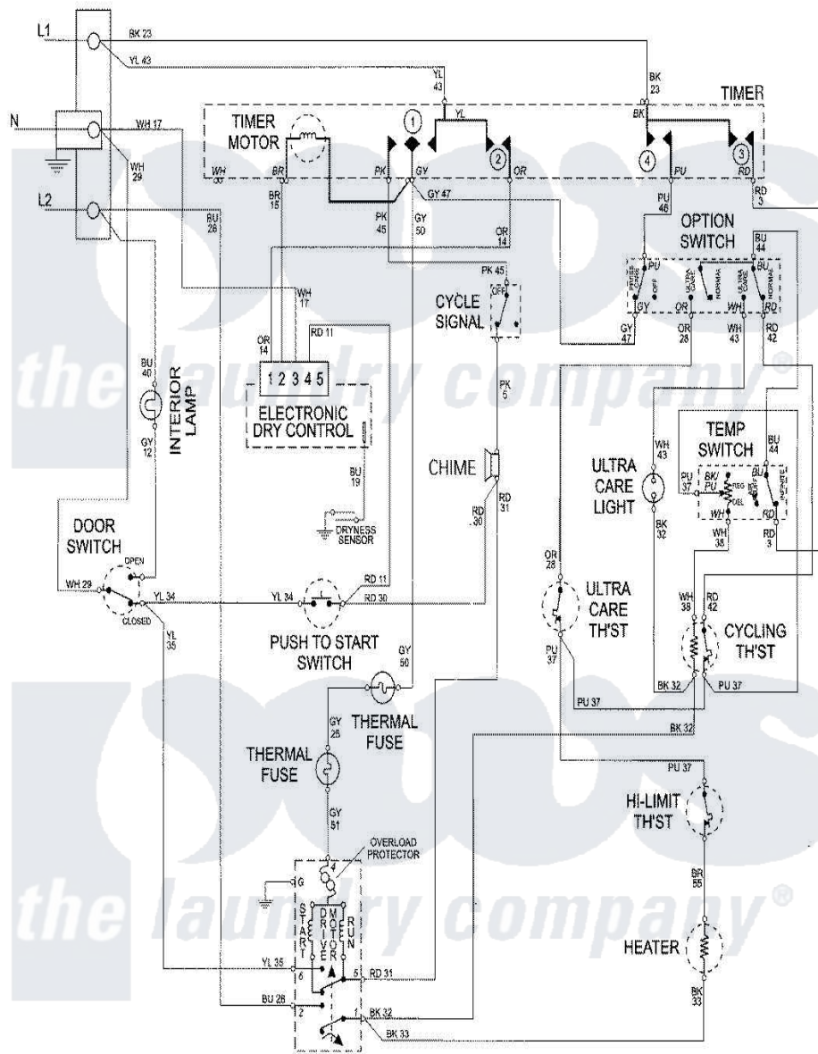
Maytag Residential Maytag MDE8500AYW Dryer Parts Parts Diagram 08 - WIRING INFORMATION Click on the part number to view part
