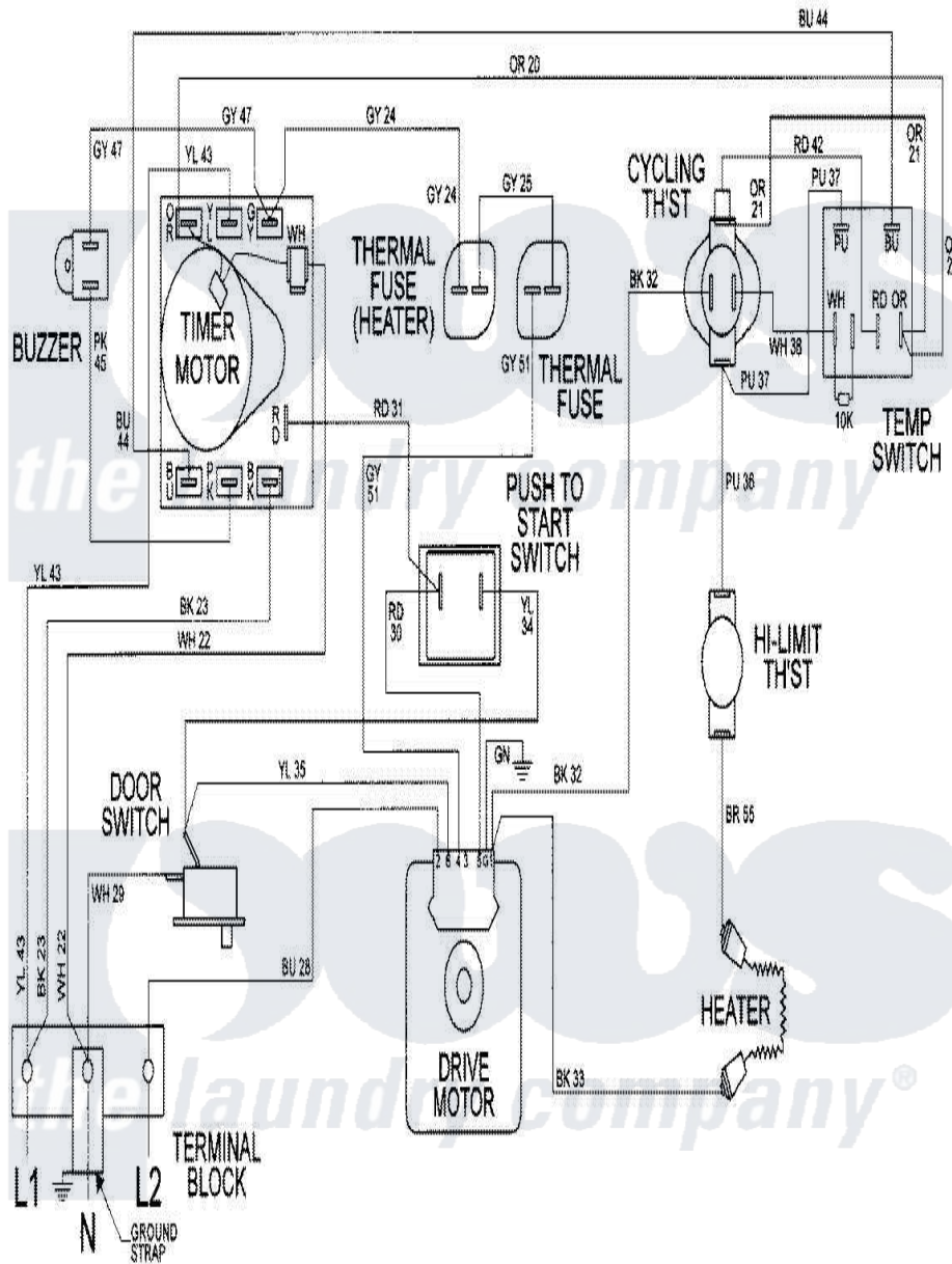
Maytag Residential Maytag MDE8506AYA Dryer Parts Parts Diagram 08 - WIRING INFORMATION Click on the part number to view part
