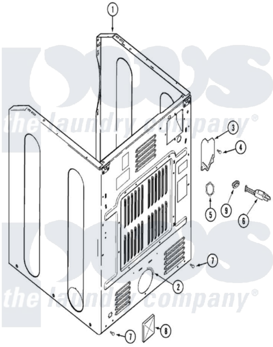
Maytag Residential Maytag MDE8600AYQ Dryer Parts Parts Diagram 02 - CABINET-REAR Click on the part number to view part
