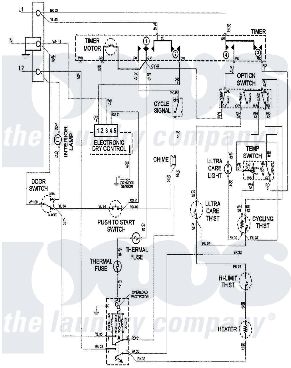
Maytag Residential Maytag MDE8600AYW Dryer Parts Parts Diagram 09 - WIRING INFORMATION Click on the part number to view part
