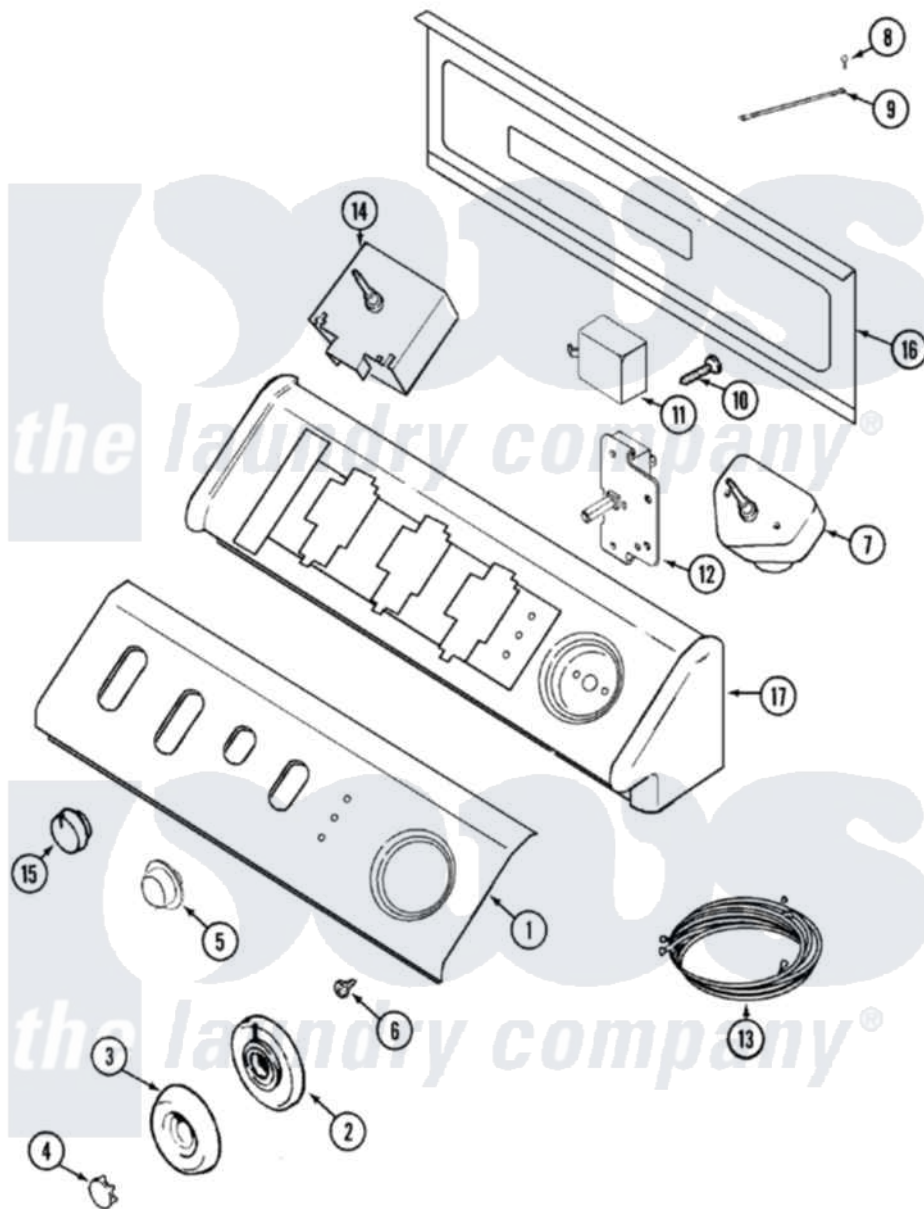
Maytag Residential Maytag MDE9306AZA Dryer Parts Parts Diagram 03 - CONTROL PANEL
