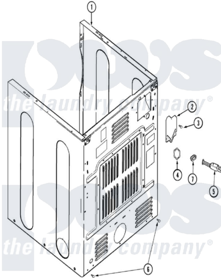
Maytag Residential Maytag MDE9706AZW Dryer Parts Parts Diagram 02 - CABINET-REAR Click on the part number to view part
