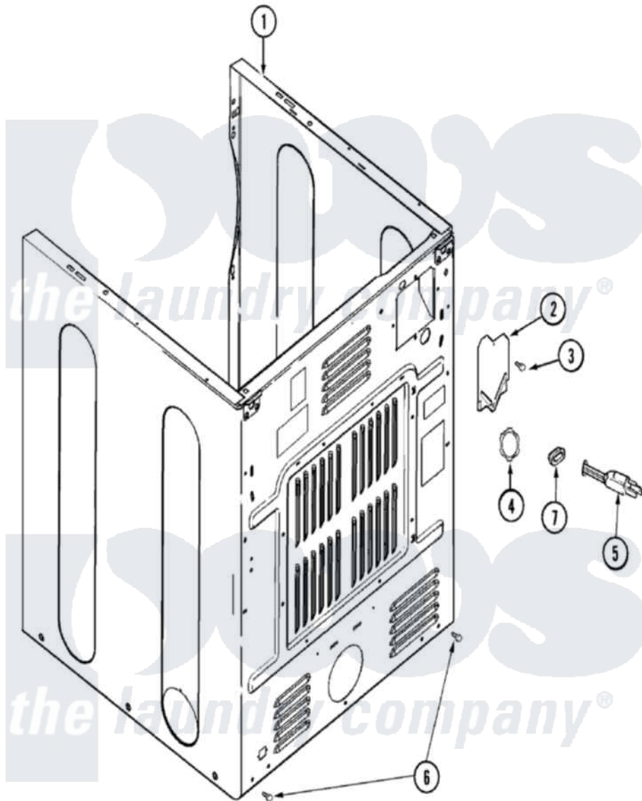
Maytag Residential Maytag MDE9766AYW Dryer Parts Parts Diagram 02 - CABINET-REAR Click on the part number to view part
