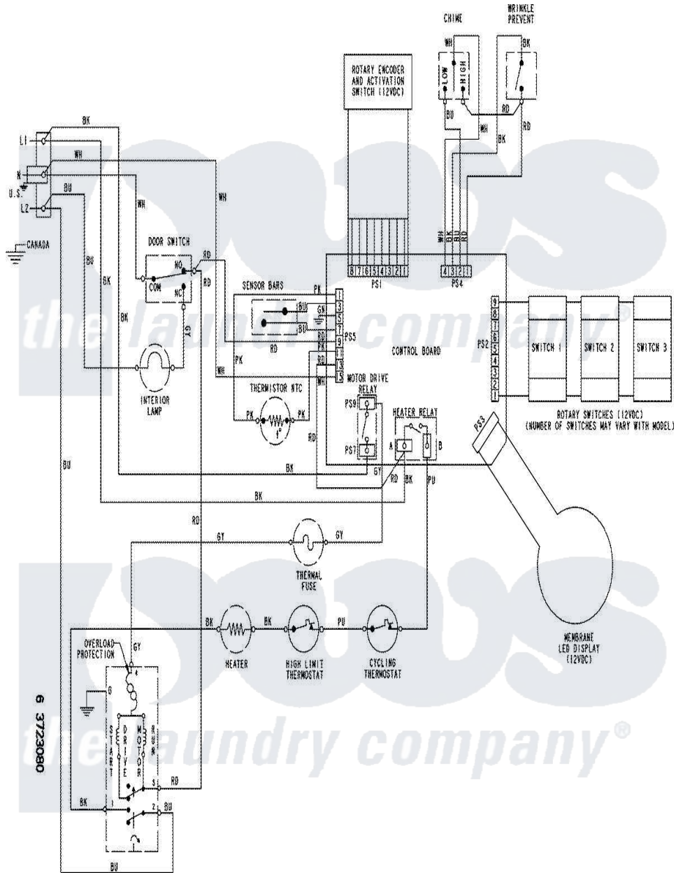
Maytag Residential Maytag MDET446AYW Dryer Parts Parts Diagram 06 - WIRING INFORMATION Click on the part number to view part
