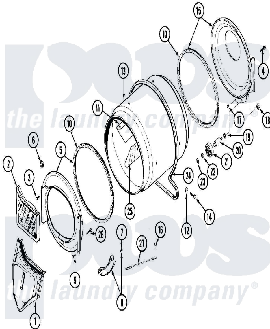
Maytag Residential Maytag MDG10PSAGW Dryer Parts Parts Diagram 06 - TUMBLER Click on the part number to view part
