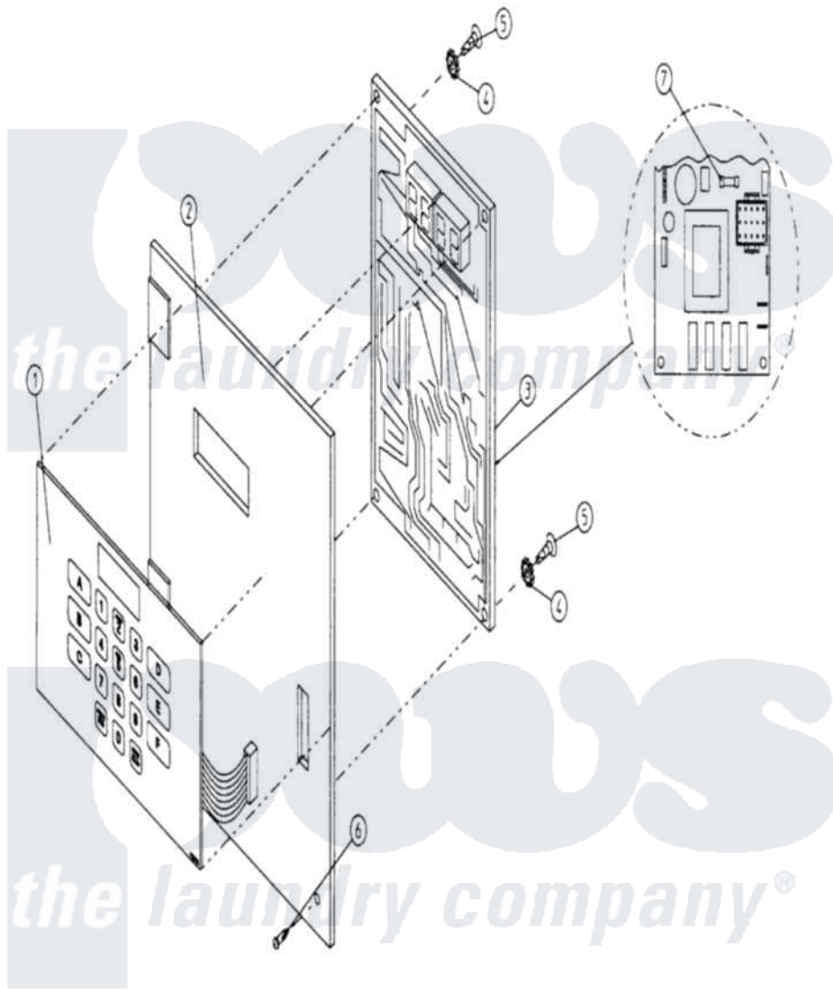
Maytag Residential Maytag MDG120P1HW Dryer Parts Diagram 01 - MICROPROCESSOR CONTROL PANEL ASSY
