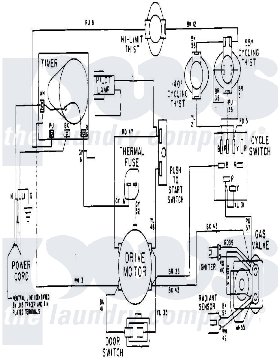
Maytag Residential Maytag MDG12MNAAW Dryer Parts Parts Diagram 07 - WIRING INFORMATION Click on the part number to view part
