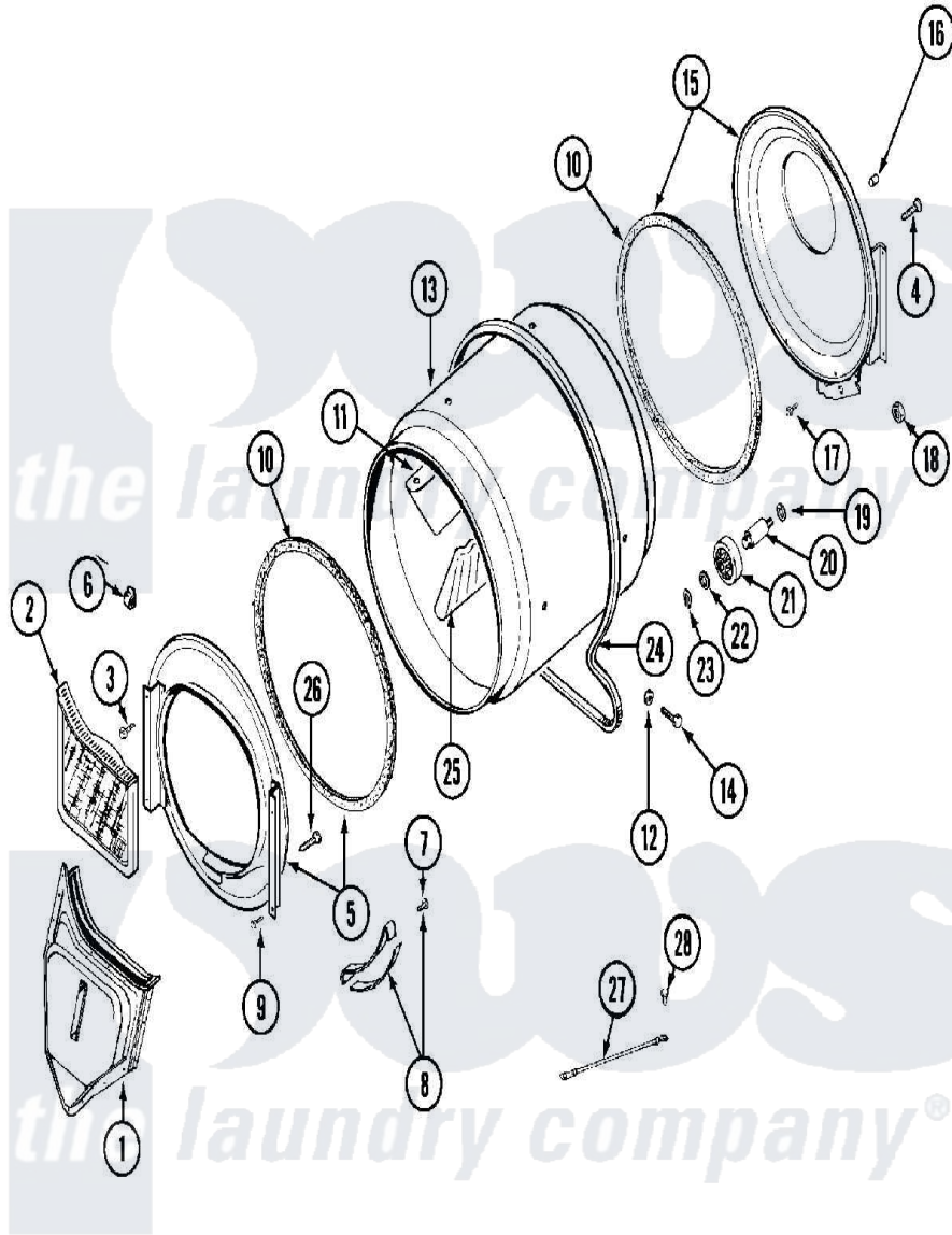
Maytag Residential Maytag MDG13CSABW Dryer Parts Parts Diagram 06 - TUMBLER Click on the part number to view part
