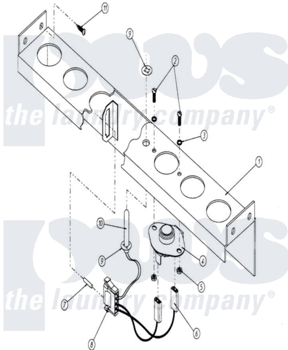
Maytag Residential Maytag MDG170P1HW Dryer Parts Parts Diagram 08 - MICROPROCESSOR TEMP. SENSOR BRKT. ASSY.
