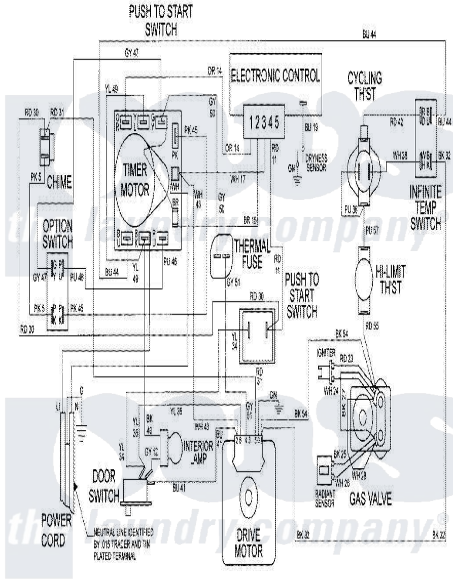
Maytag Residential Maytag MDG3000AWA Dryer Parts Parts Diagram 09 - WIRING INFORMATION Click on the part number to view part
