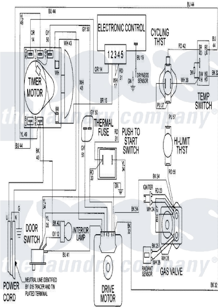
Maytag Residential Maytag MDG4000BWQ Dryer Parts Parts Diagram 08 - WIRING INFORMATION Click on the part number to view part
