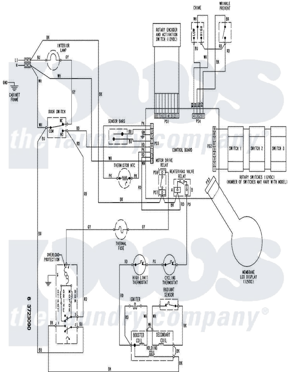
Maytag Residential Maytag MDG4806AWW Dryer Parts Parts Diagram 06 - WIRING INFORMATION Click on the part number to view part
