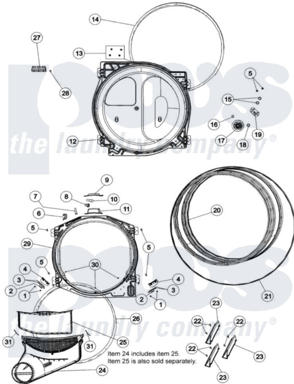
Maytag Residential Maytag MDG508DAWK Dryer Parts Parts Diagram 05 - TUMBLER Click on the part number to view part
