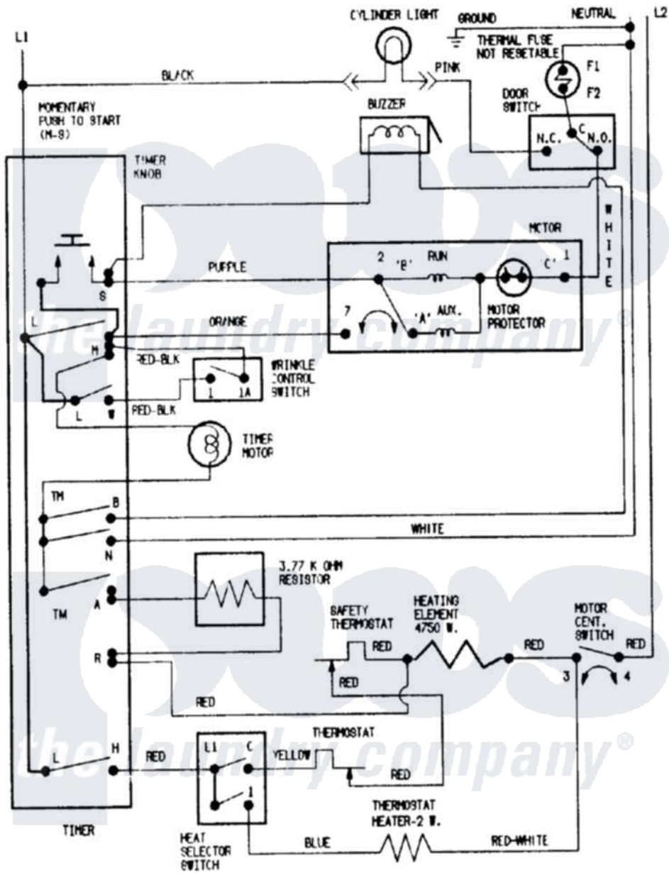
Maytag Residential Maytag MDG508DAWK Dryer Parts Parts Diagram 06 - WIRING INFORMATION Click on the part number to view part
