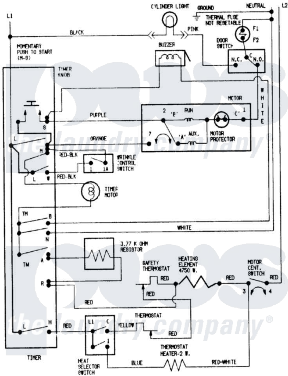
Maytag Residential Maytag MDG508DAWW Dryer Parts Parts Diagram 06 - WIRING INFORMATION Click on the part number to view part
