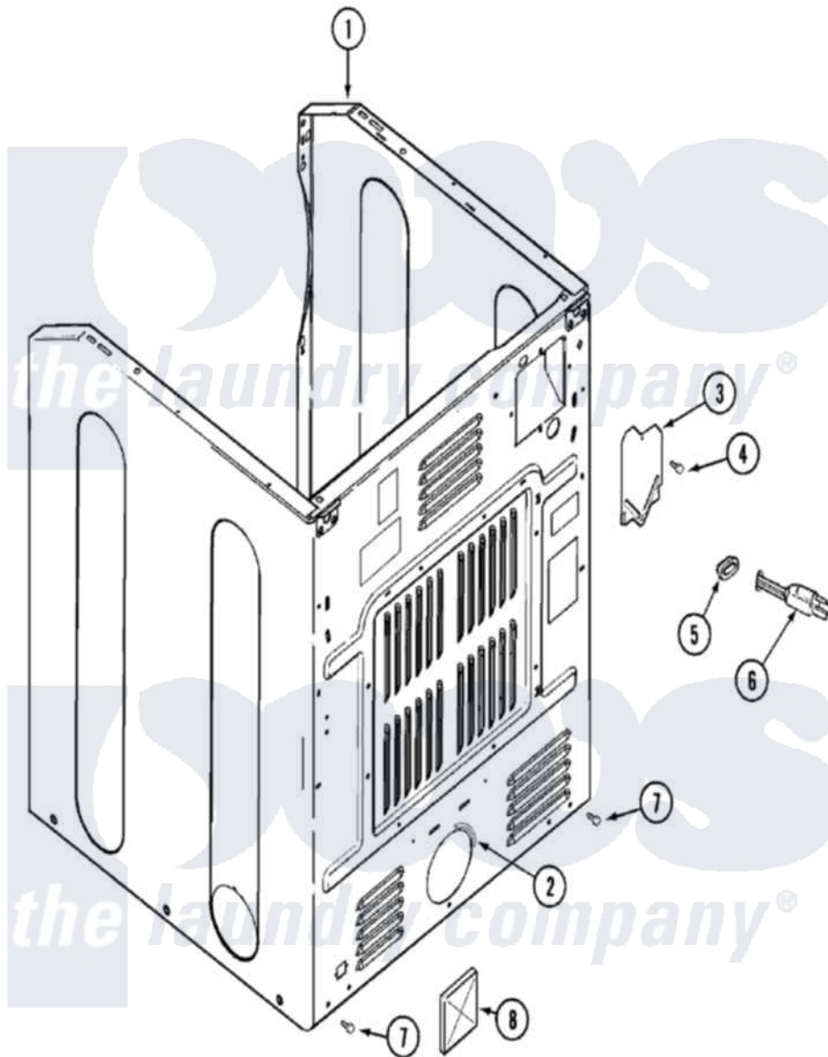
Maytag Residential Maytag MDG5500AWQ Dryer Parts Parts Diagram 01 - CABINET-REAR Click on the part number to view part
