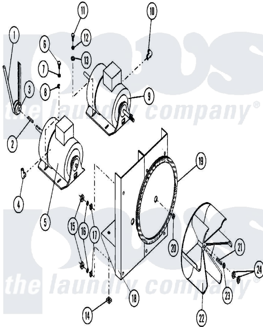
Maytag Residential Maytag MDG75PN2VW Dryer Parts Parts Diagram 14 - MOTOR & MOUNT ASSEMBLY (PN2V) Click on the part number to view part
