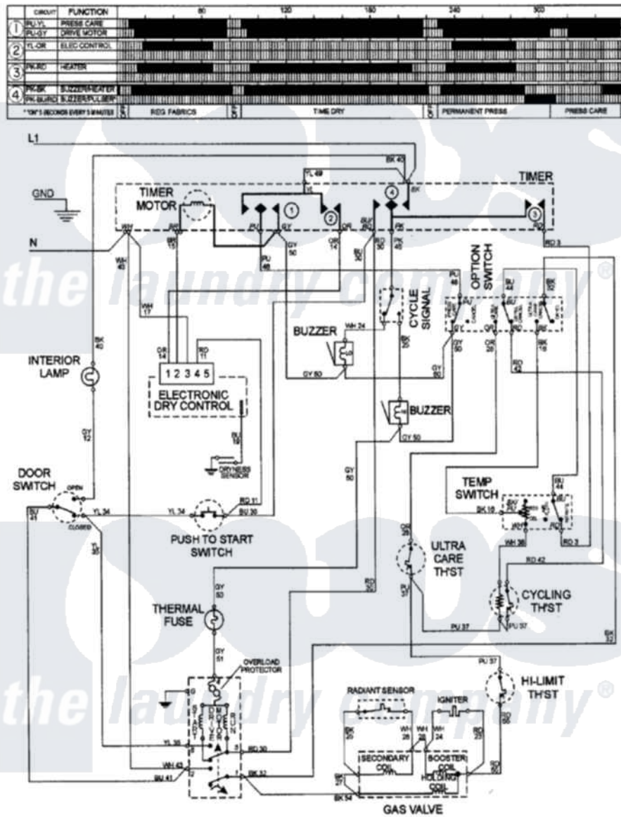
Maytag Residential Maytag MDG8058BWQ Dryer Parts Parts Diagram 05 - WIRING INFORMATION Click on the part number to view part
