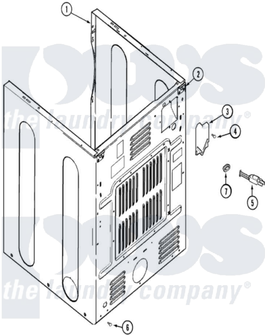
Maytag Residential Maytag MDG8426AAW Dryer Parts Parts Diagram 02 - CABINET-REAR Click on the part number to view part
