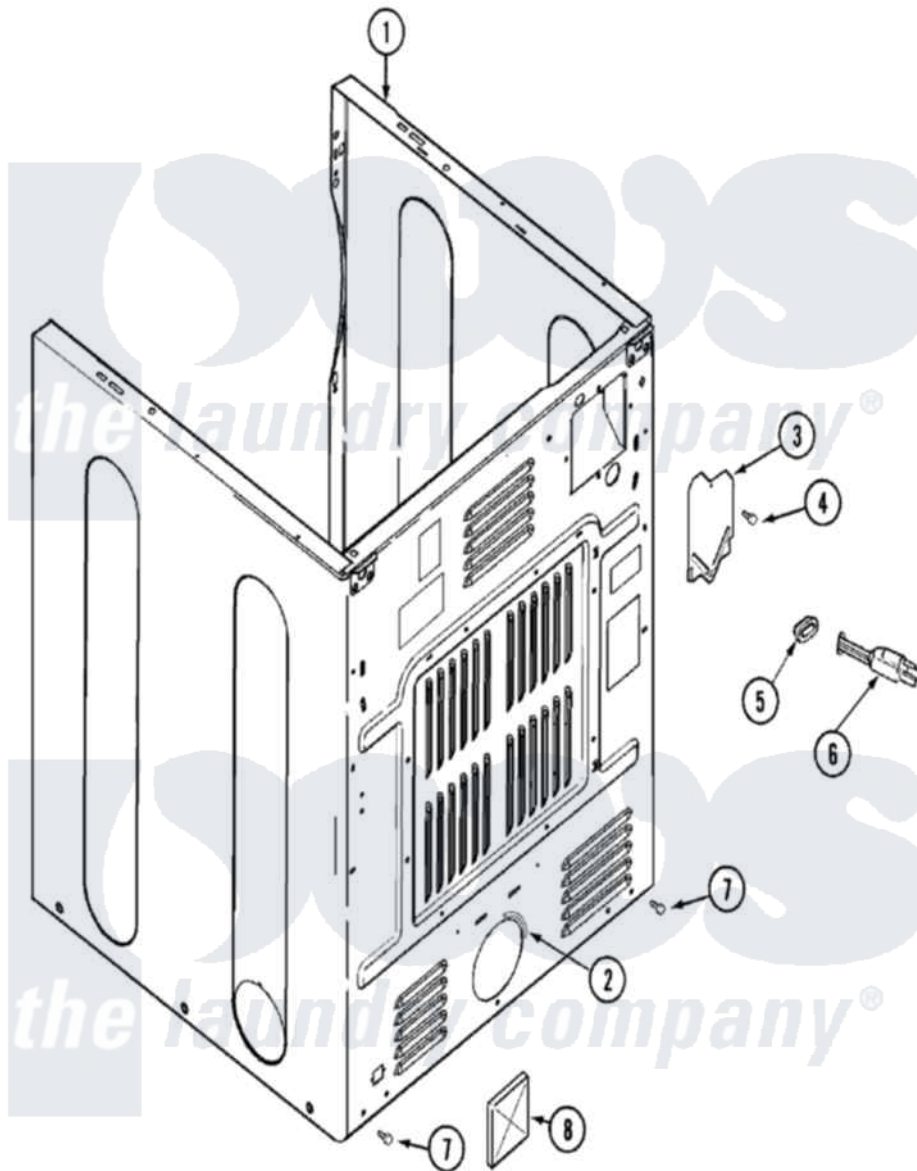
Maytag Residential Maytag MDG9360BWW Dryer Parts Parts Diagram 02 - CABINET-REAR Click on the part number to view part
