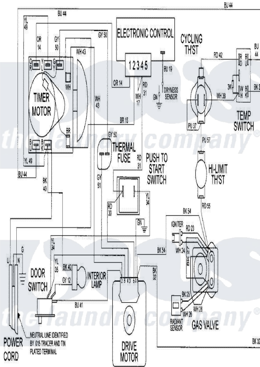
Maytag Residential Maytag MDG9766AWW Dryer Parts Parts Diagram 08 - WIRING INFORMATION Click on the part number to view part
