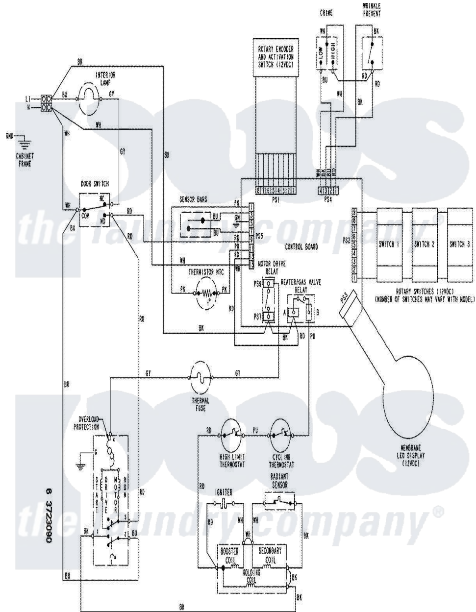
Maytag Residential Maytag MDGT446AWW Dryer Parts Parts Diagram 06 - WIRING INFORMATION Click on the part number to view part
