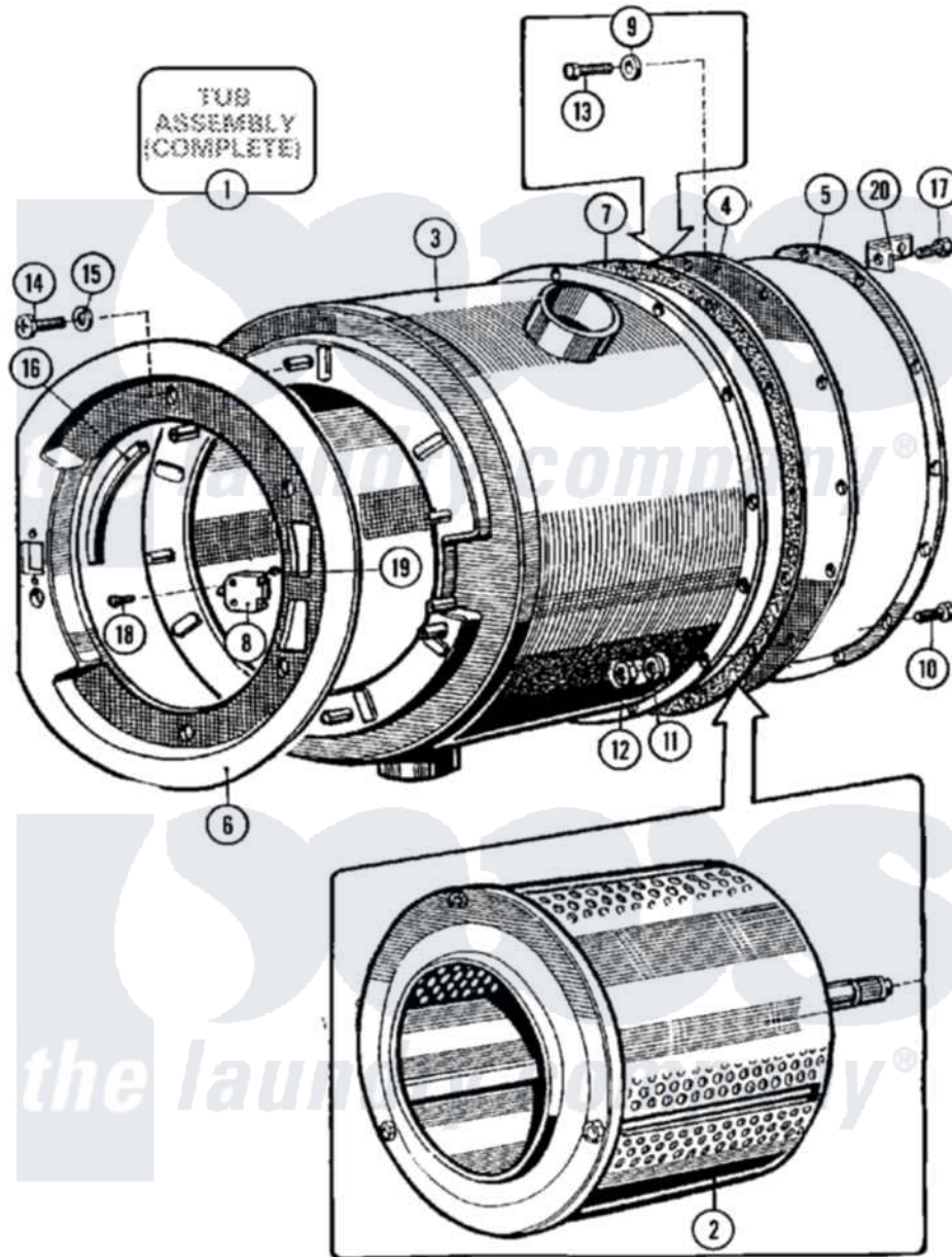
Maytag Residential Maytag MFR18MCAAS Washer Parts Parts Diagram 08 - BASKET & OUTER SHELL ASSY. (SERIES 10)
