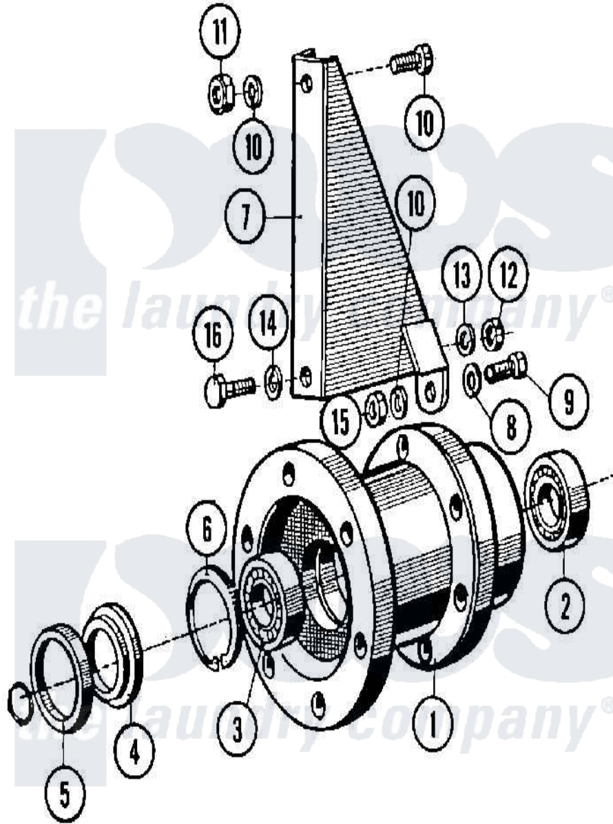
Maytag Residential Maytag MFR18MCAAS Washer Parts Parts Diagram 09 - BEARINGS & TRUNNION ASSY. (SERIES 10)
