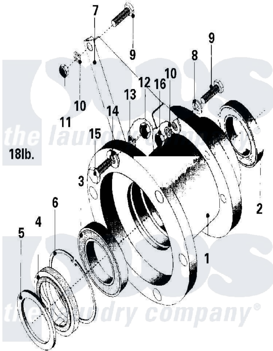
Maytag Residential Maytag MFR18MCAVS Washer Parts Parts Diagram 25 - BEARINGS & TRUNNION ASSY. (SERIES 11)
