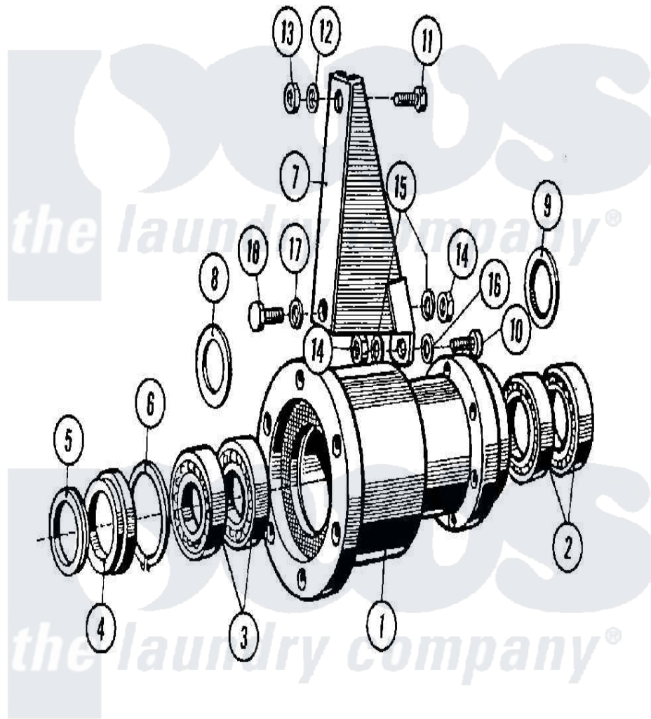
Maytag Residential Maytag MFR25PCATS Washer Parts Parts Diagram 08 - BEARINGS & TRUNNION ASSY. (SERIES 10)
