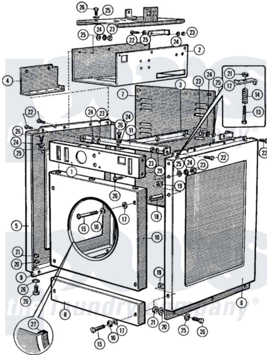
Maytag Residential Maytag MFR25PCATS Washer Parts Parts Diagram 12 - CABINET (SERIES 10) Click on the part number to view part
