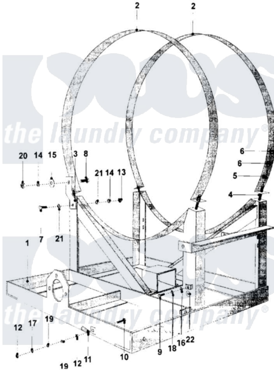
Maytag Residential Maytag MFR25PCATS Washer Parts Parts Diagram 22 - BASE FRAME (SERIES 11) Click on the part number to view part
