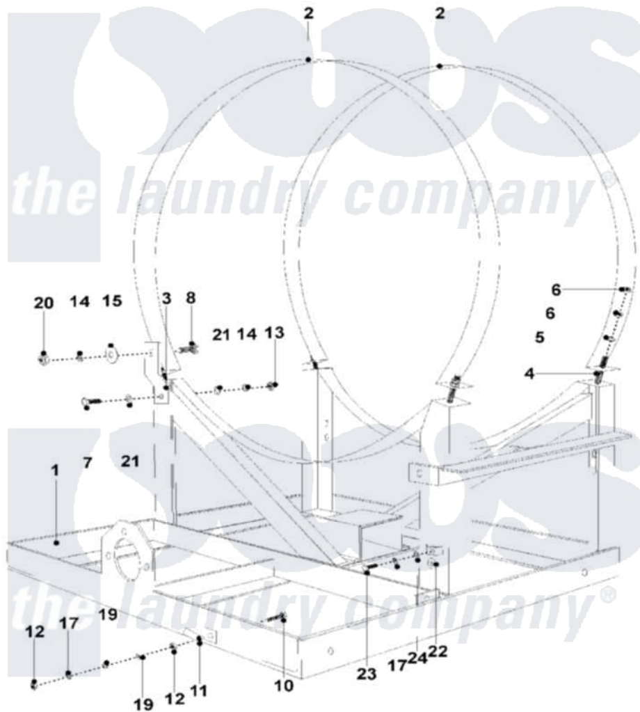
Maytag Residential Maytag MFR25PDATS Washer Parts Parts Diagram 01 - BASE FRAME Click on the part number to view part
