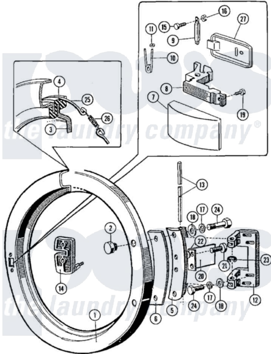
Maytag Residential Maytag MFR35PDAVS Washer Parts Parts Diagram 07 - DOOR Click on the part number to view part
