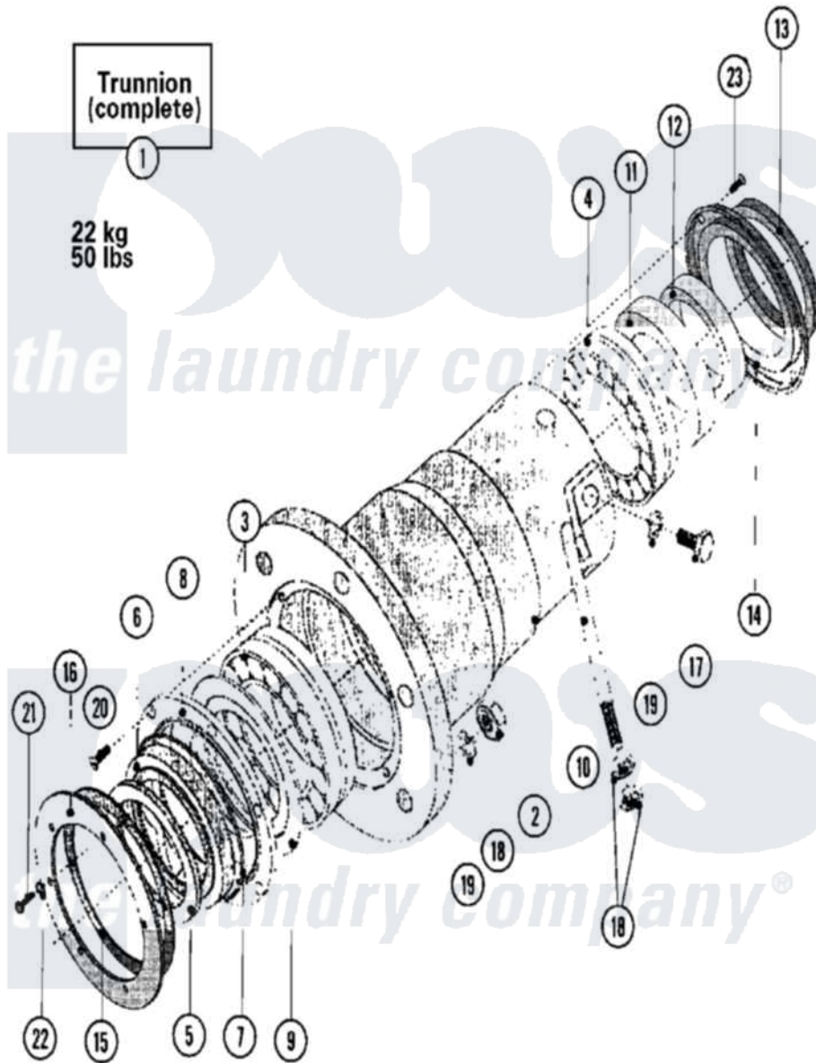
Maytag Residential Maytag MFR50PCATS Washer Parts Parts Diagram 25 - BEARINGS & TRUNNION ASSEMBLY (SERIES 11)
