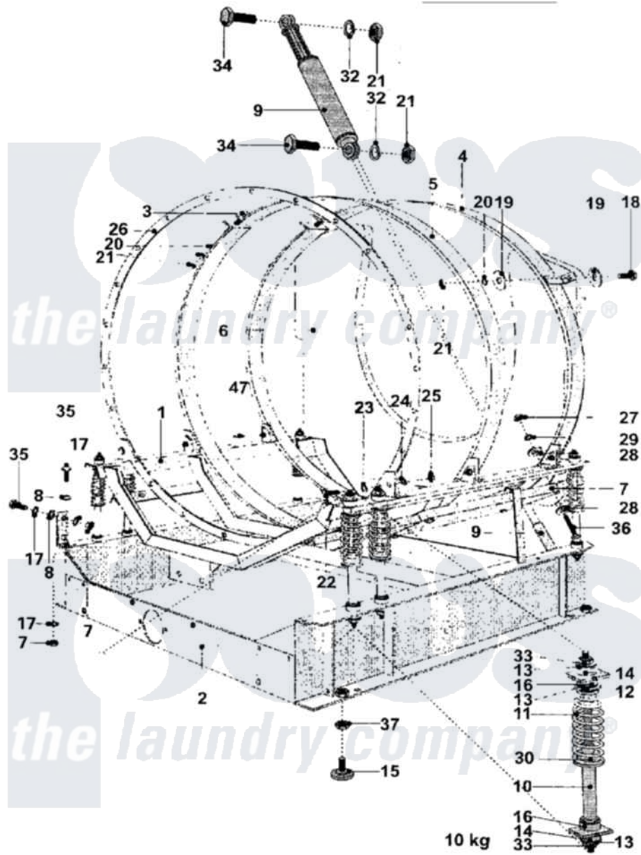
Maytag Residential Maytag MFS25PNAVS Washer Parts Parts Diagram 01 - FRAME Click on the part number to view part
