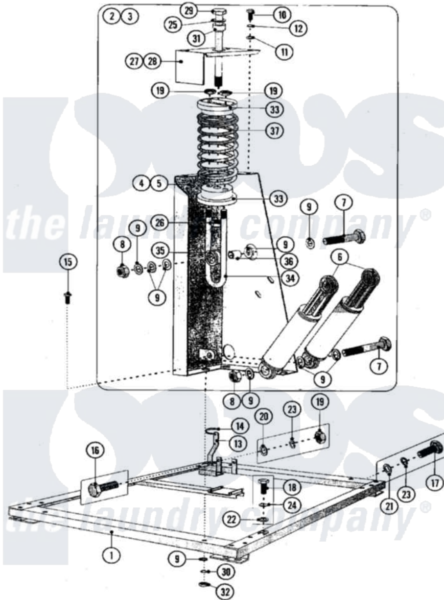
Maytag Residential Maytag MFS50PNAVS Washer Parts Parts Diagram 01 - BASE Click on the part number to view part
