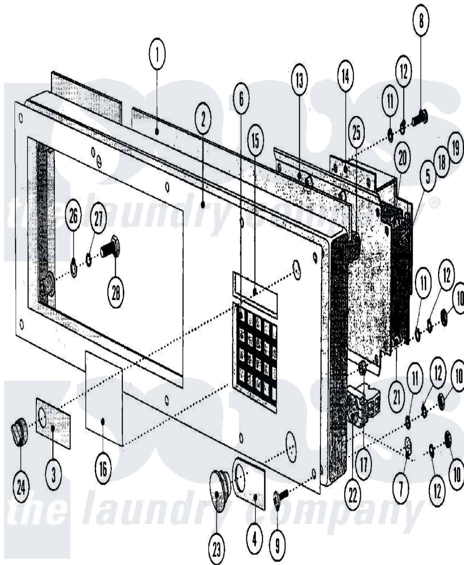
Maytag Residential Maytag MFS50PNAVS Washer Parts Parts Diagram 12 - CONTROL PANEL Click on the part number to view part
