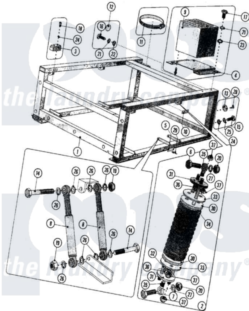
Maytag Residential Maytag MFS75PNAVS Washer Parts Parts Diagram 01 - BASE Click on the part number to view part
