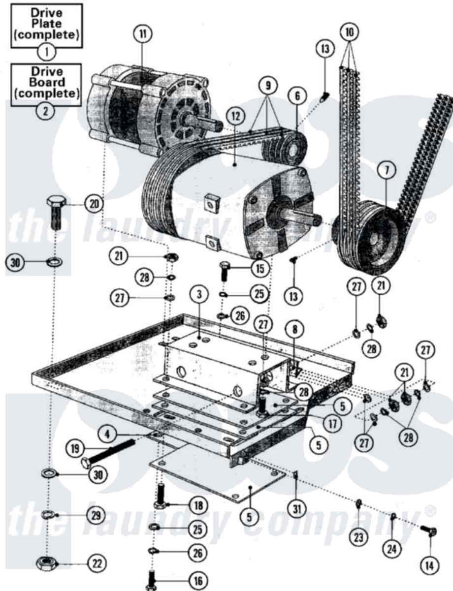
Maytag Residential Maytag MFS75PNAVS Washer Parts Parts Diagram 07 - MOTOR & BASKET PULLEY Click on the part number to view part
